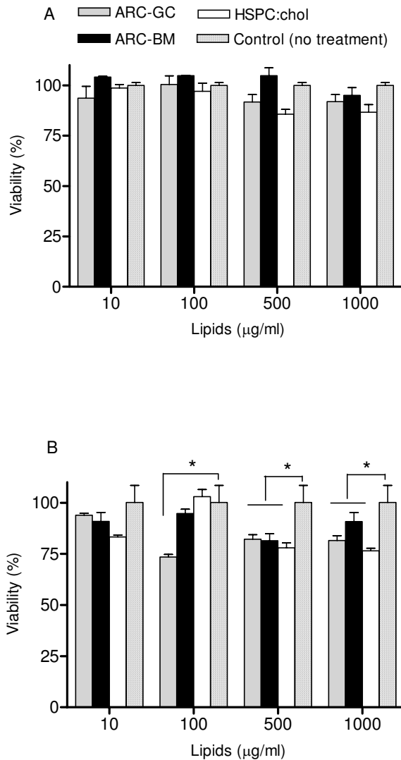
Figure 3 Viability of Vero (A) and J-774 cells (B) upon 24 h incubation with ARC-GC, ARC-BM or HSPC:cholesterol liposomes, as function of concentration. Values represent the average of triplicates \pm S.D. ANOVA, * p < 0.05 .
